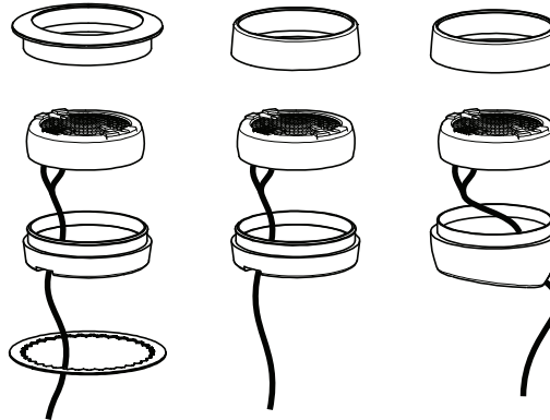
Flush Mount
